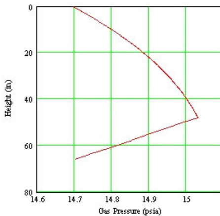
Gas injection increases solids flow rate to 280 lb/min
